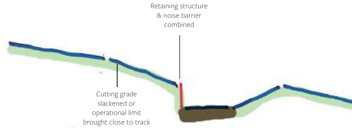
1A: Alternative Trackside Barrier
