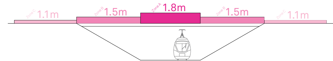
Overbridge parapet: containment heights (Source HS2 Standard Parapets documents March 2017)
