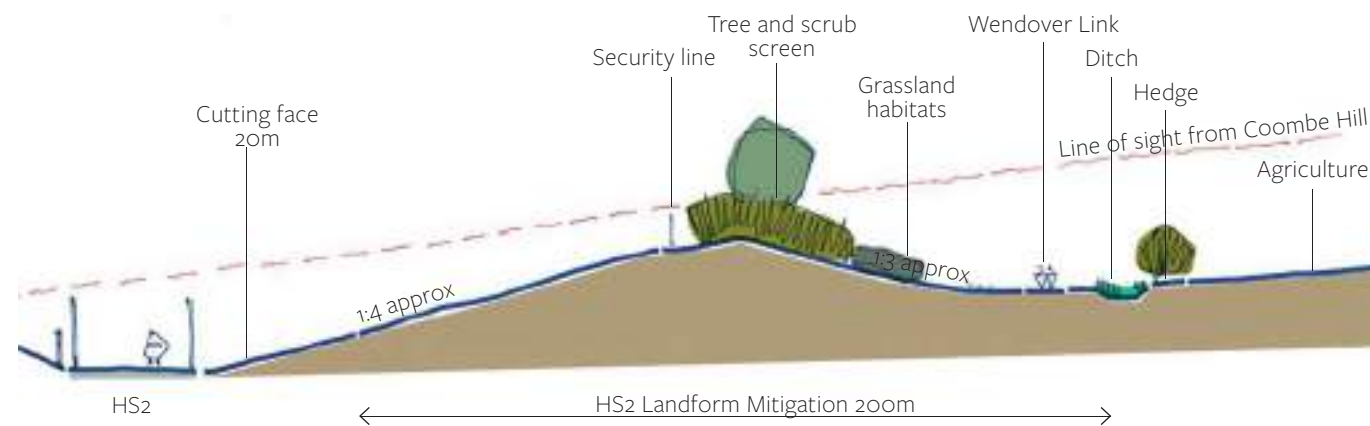
Wendover Link North, typical section: Option #1 Maximising Green Infrastructure
